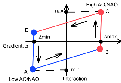
Figure 1. Hypothesized behavior of the Arctic–GIN Sea climate system. Abscissa is the between-basin gradient of SAT or dynamic height. Ordinate is the intensity of interaction between the basins, either FW or heat flux. Blue segments denote weak interaction and red segments intense interaction.
